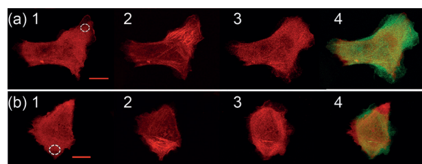
Figure 4. Localized recruitment of cofilin induces protrusive behavior. a) Localized illumination of S3A.S120ACof-Cry2-mCh/LifeAct-Cib-GFP-containing MTLn3 cells results in lamellipodia formation in the illuminated region, whereas b) localized illumination in control cells (Cry2-mCh/LifeAct-Cib-GFP) has little effect. 1) Pre-illumination, 2) 10 s (note the recruitment of cofilin to F-actin fibers) and 3) 8 min after illumination. The illumination site is highlighted in (1). 4) Cell protrusion (green) and retraction (red). Significant protrusive activity is observed in (a)(1) at the illumination site, whereas very little change is observed in (b)(4). Scale bar = 10 \mu\text{m} .
